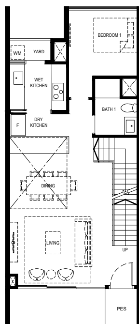
1st Storey
